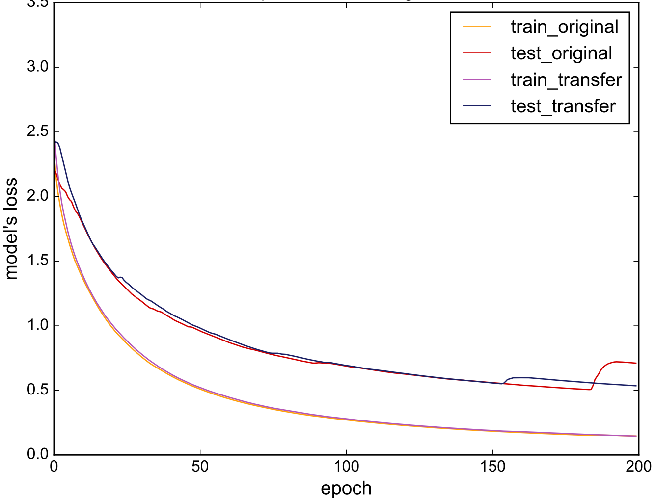
Source: ShapeletSim - Target: FacesUCR
