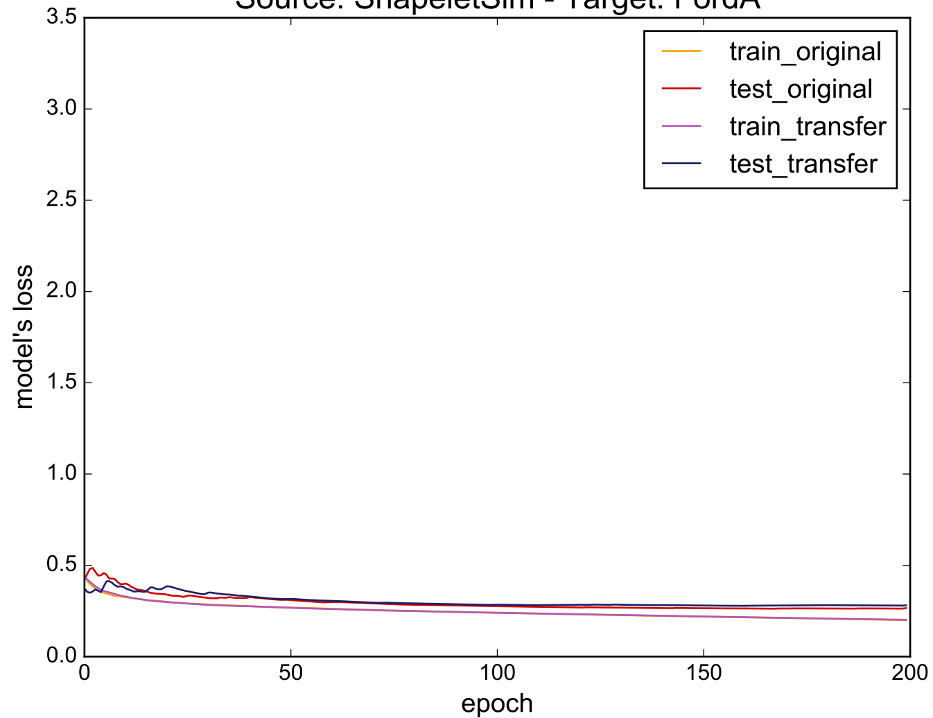
Source: ShapeletSim - Target: FordA
