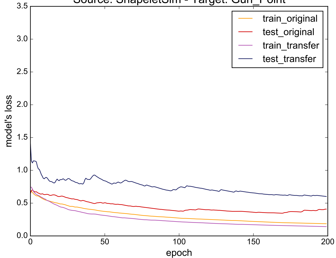
Source: ShapeletSim - Target: Gun_Point
