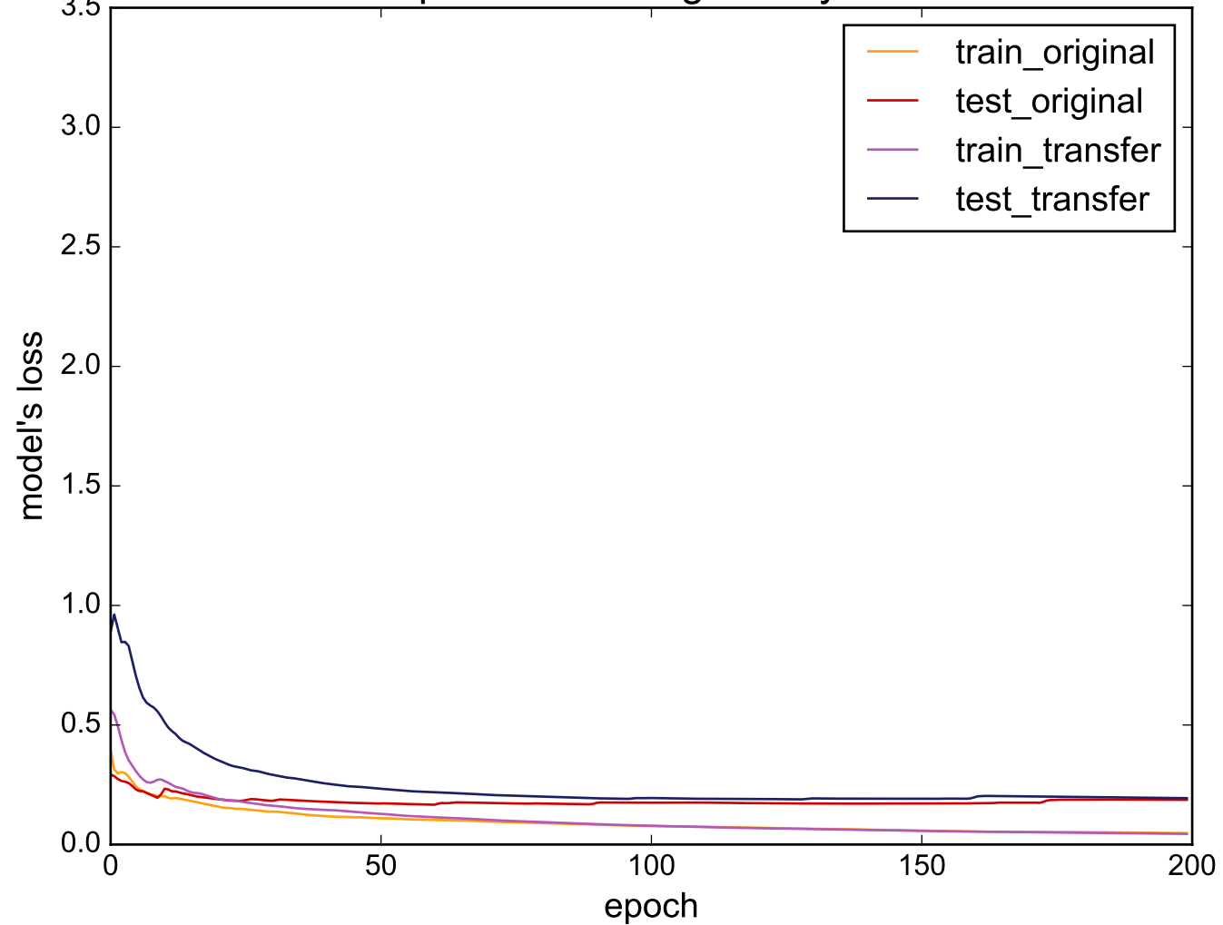
Source: ShapeletSim - Target: ItalyPowerDemand
