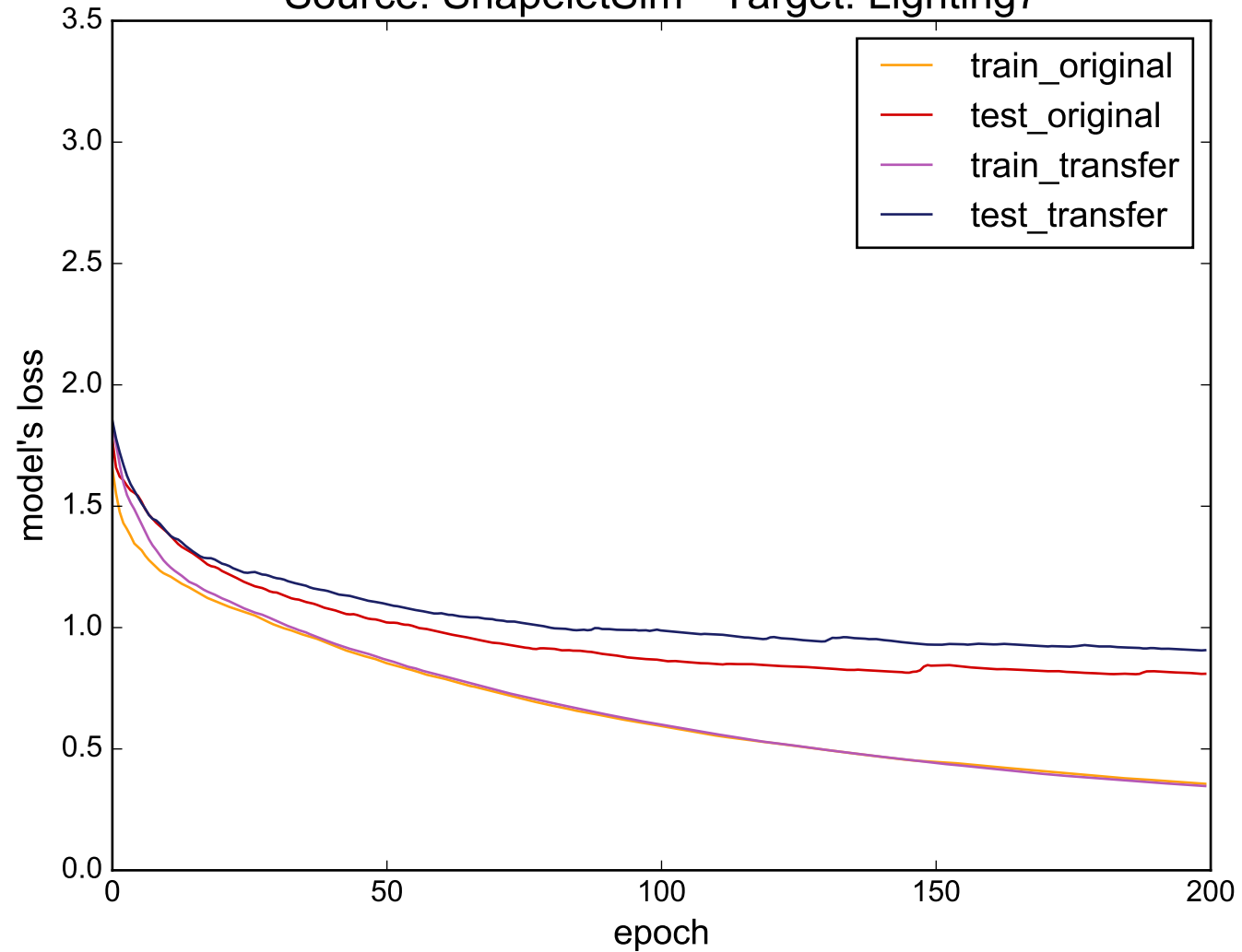
Source: ShapeletSim - Target: Lighting7
