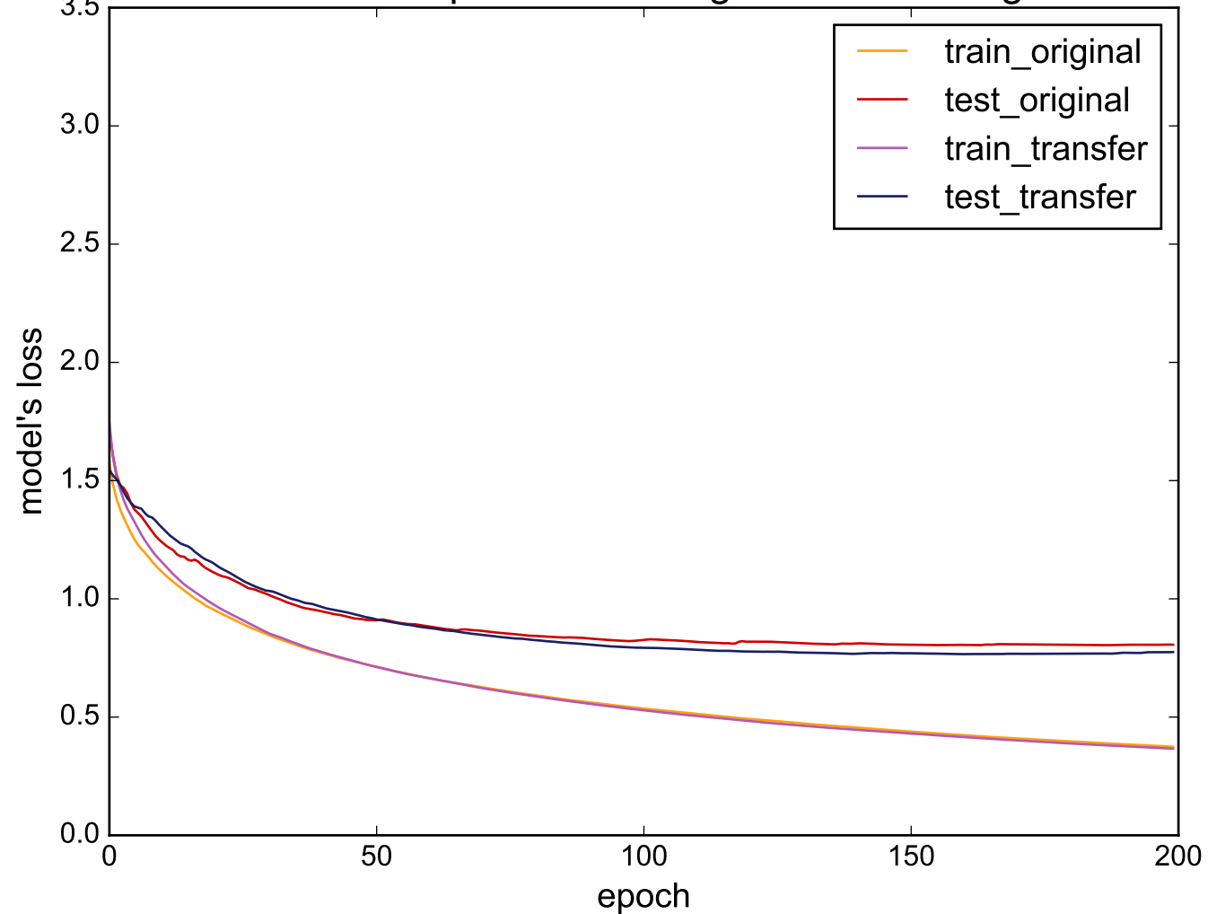
Source: ShapeletSim - Target: MedicalImages
