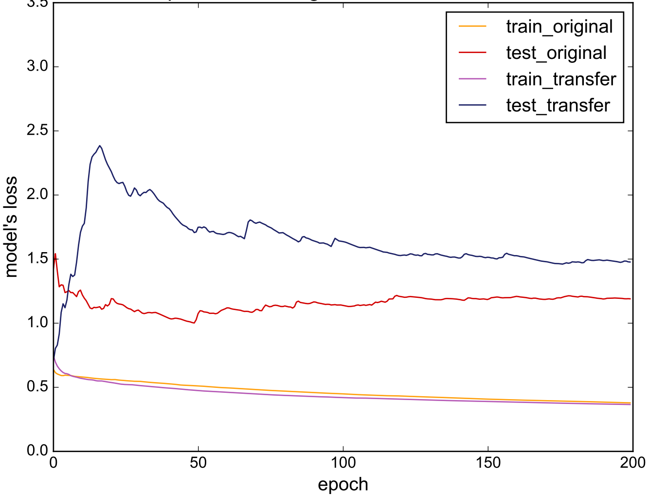
Source: ShapeletSim - Target: MiddlePhalanxOutlineCorrect
