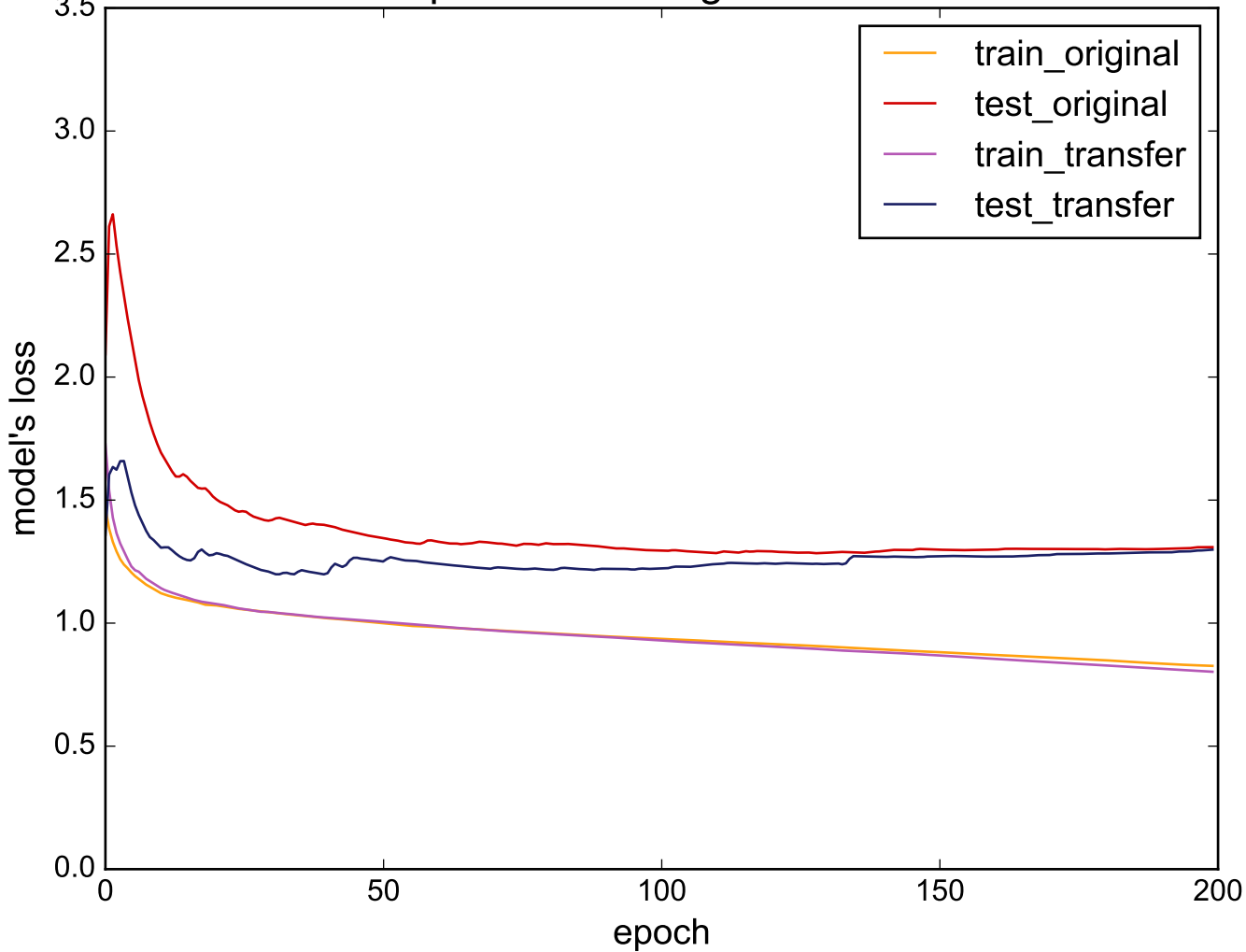
Source: ShapeletSim - Target: MiddlePhalanxTW
