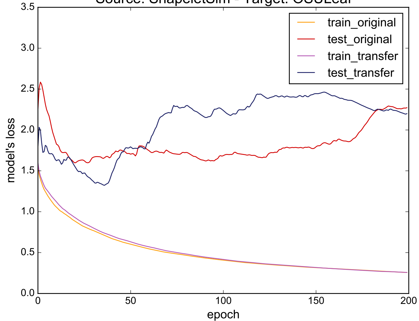
Source: ShapeletSim - Target: OSULeaf
