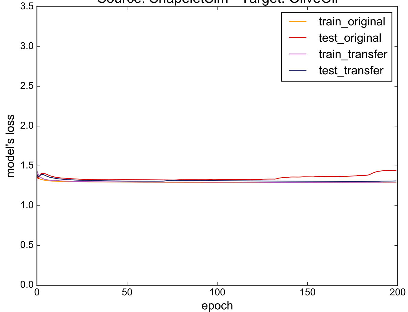
Source: ShapeletSim - Target: OliveOil
