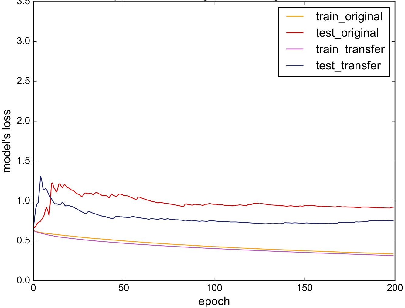
Source: ShapeletSim - Target: PhalangesOutlinesCorrect
