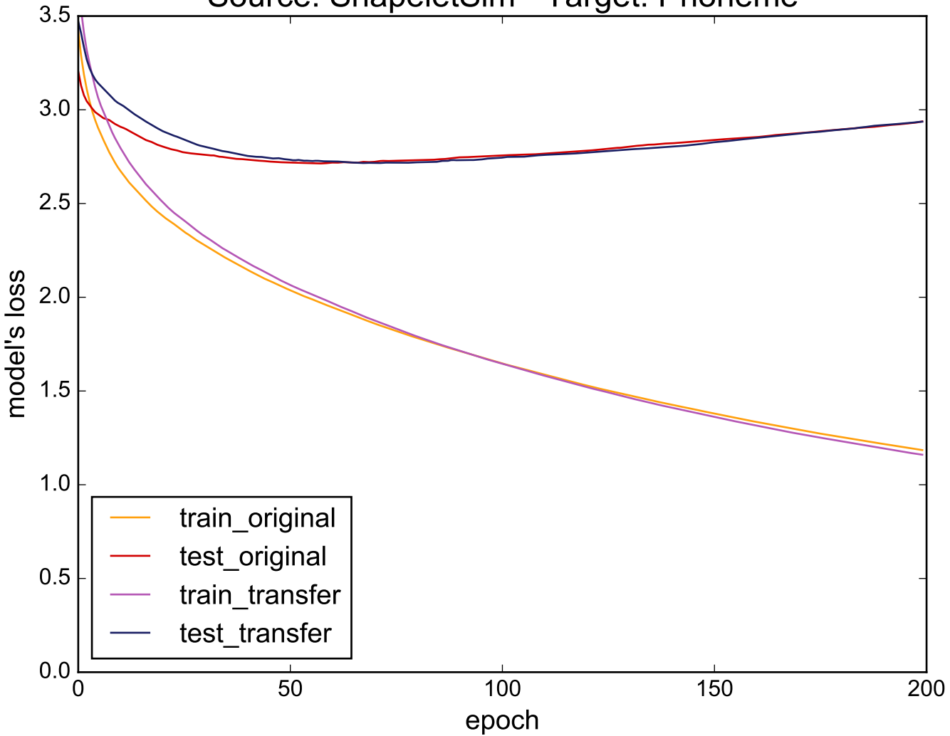
Source: ShapeletSim - Target: Phoneme
