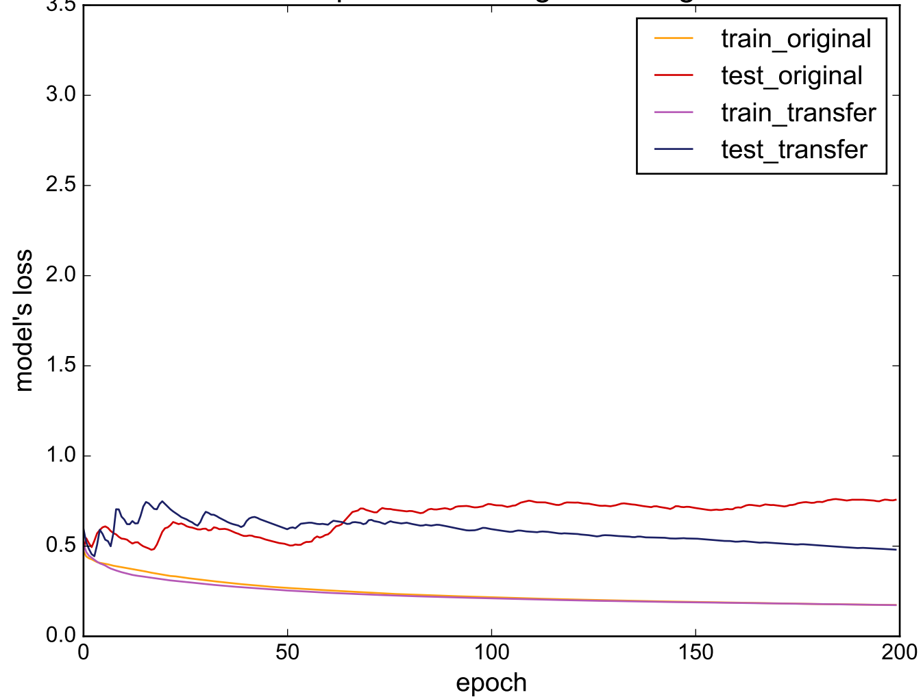
Source: ShapeletSim - Target: StarLightCurves
