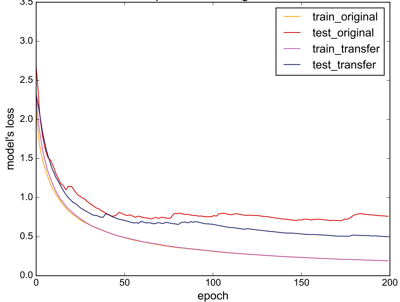
Source: ShapeletSim - Target: SwedishLeaf
