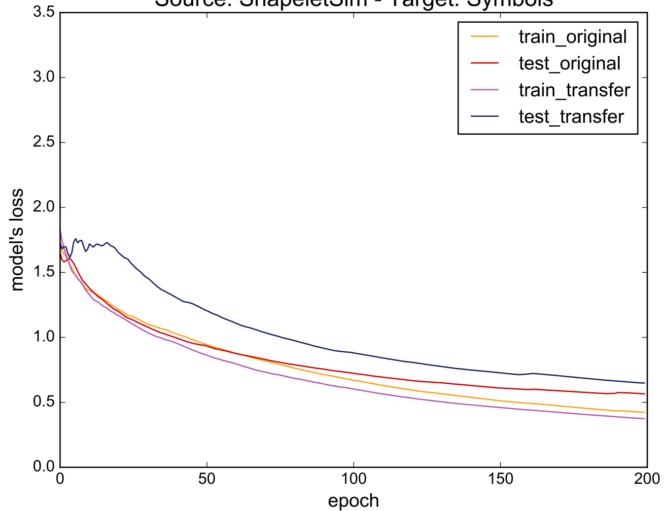
Source: ShapeletSim - Target: Symbols
