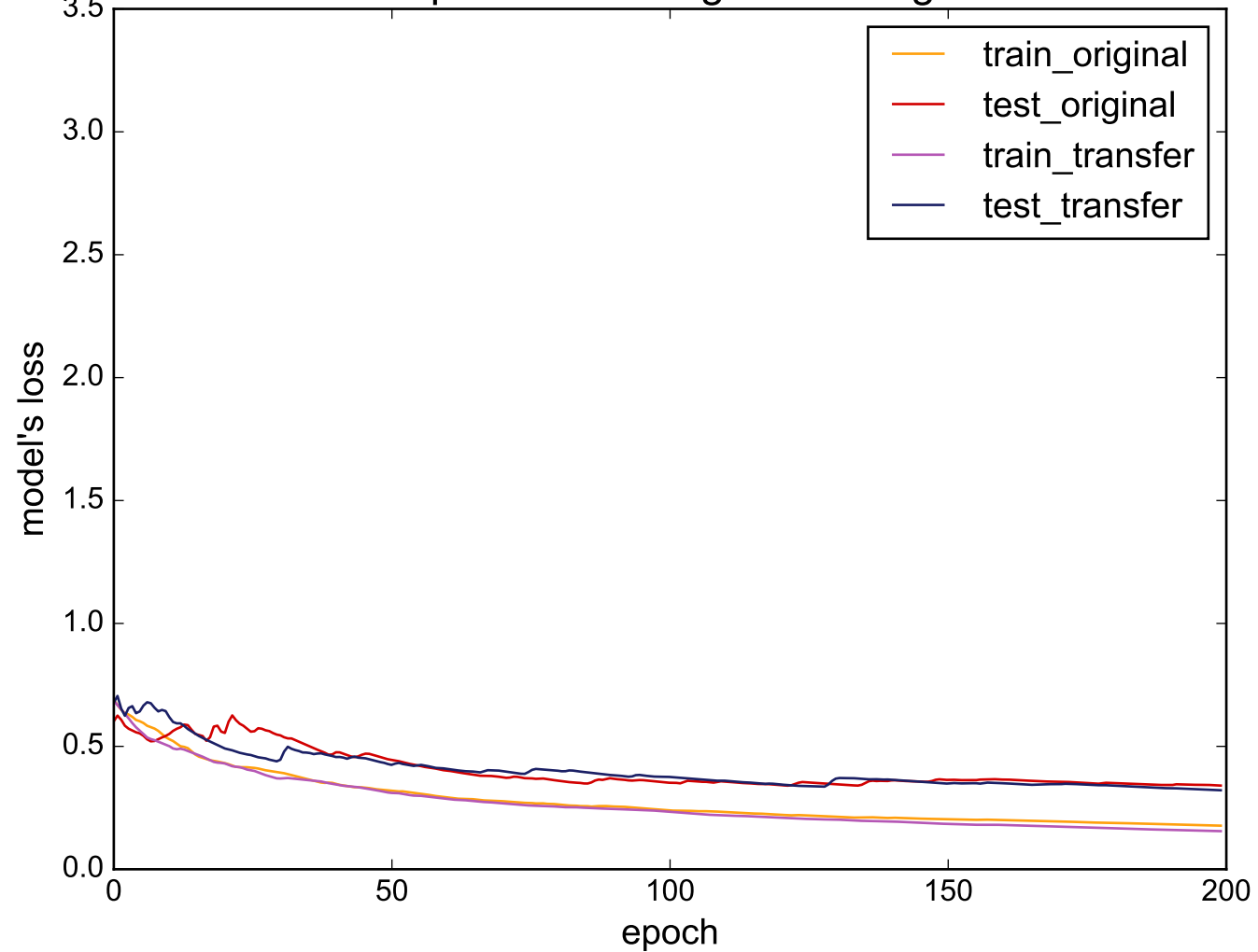
Source: ShapeletSim - Target: ToeSegmentation1
