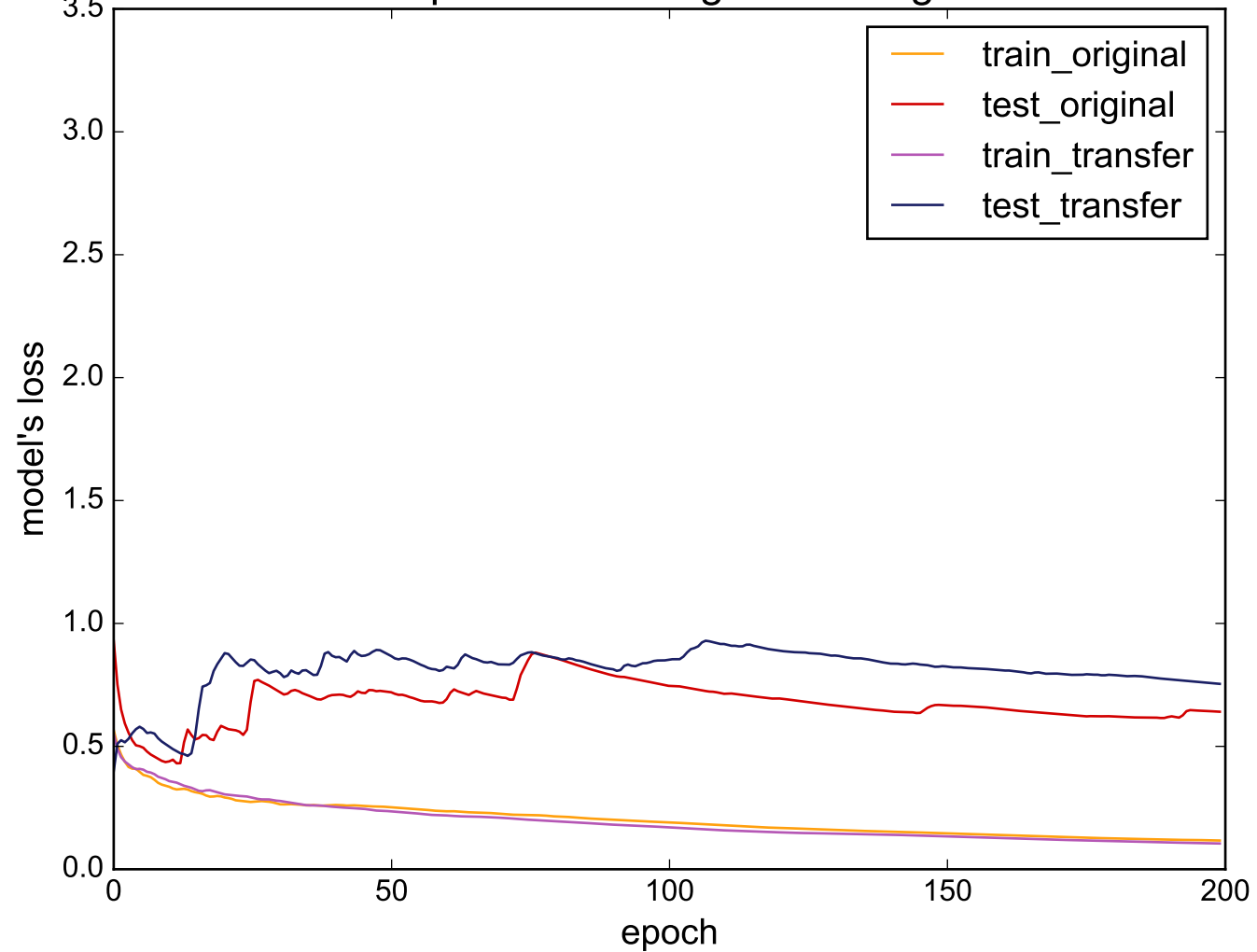
Source: ShapeletSim - Target: ToeSegmentation2
