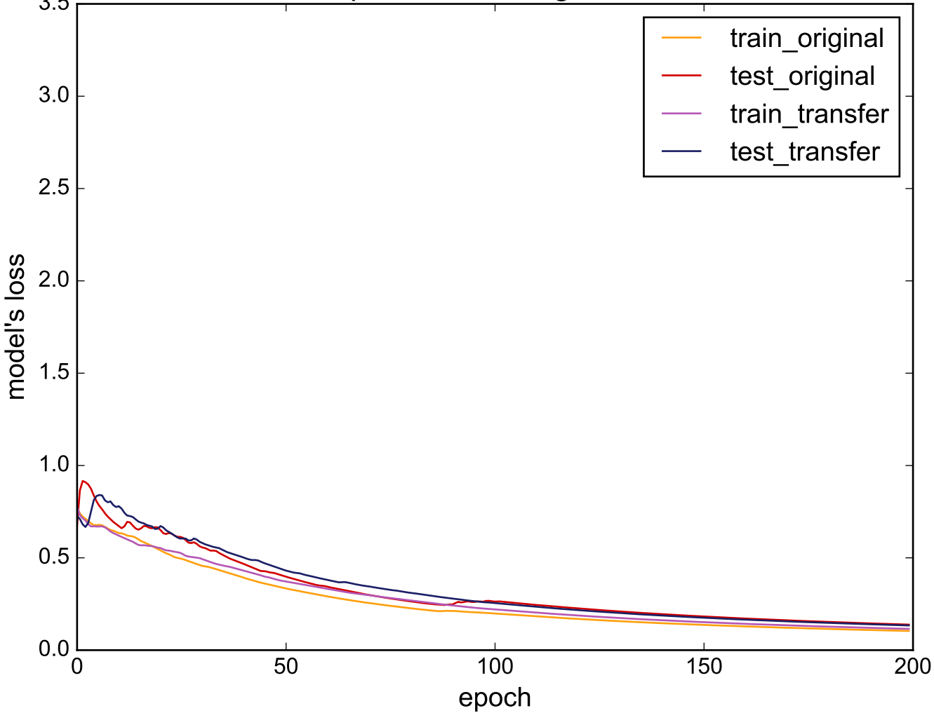
Source: ShapeletSim - Target: TwoLeadECG
