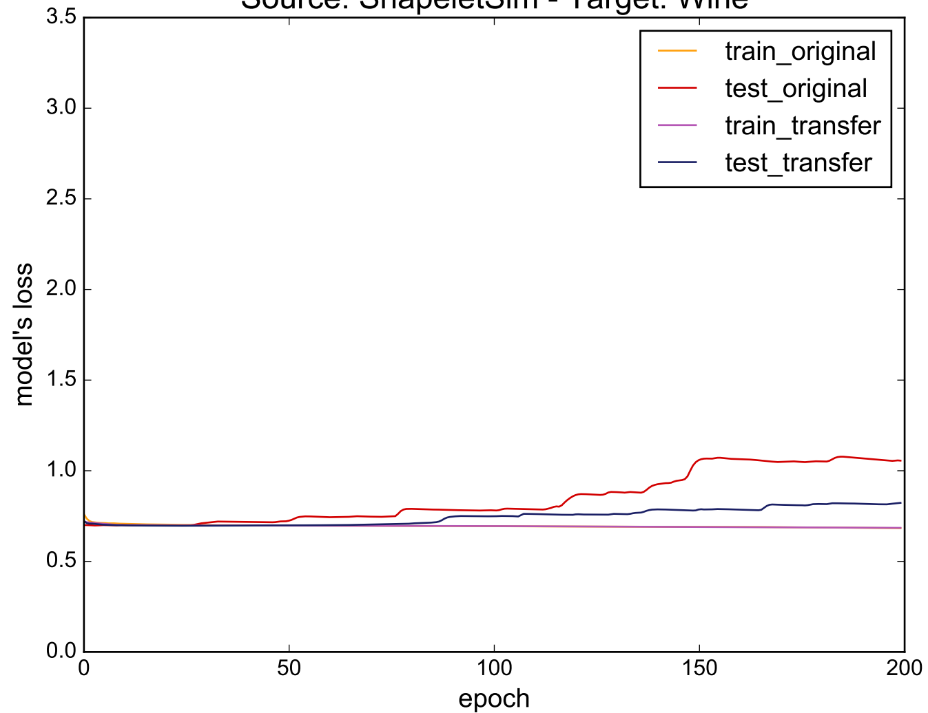
Source: ShapeletSim - Target: Wine
