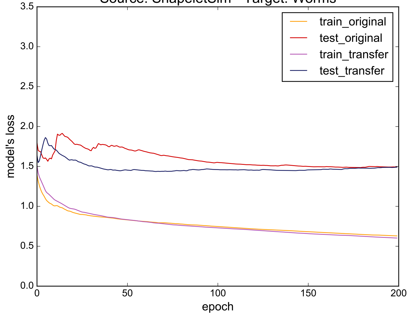
Source: ShapeletSim - Target: Worms
