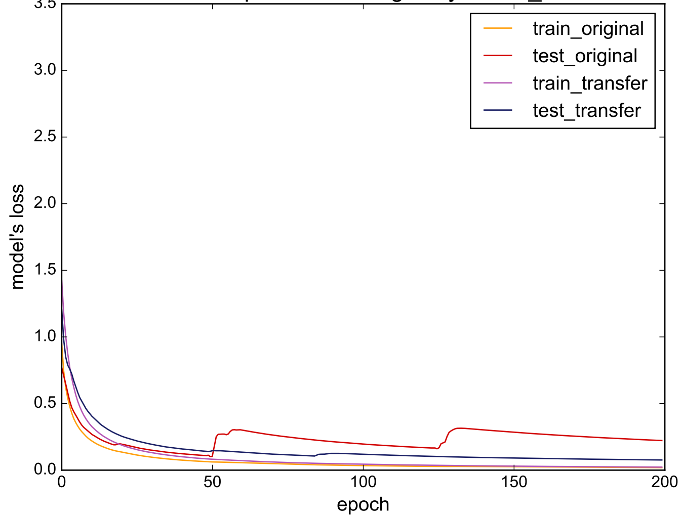
Source: ShapeletSim - Target: synthetic_control
