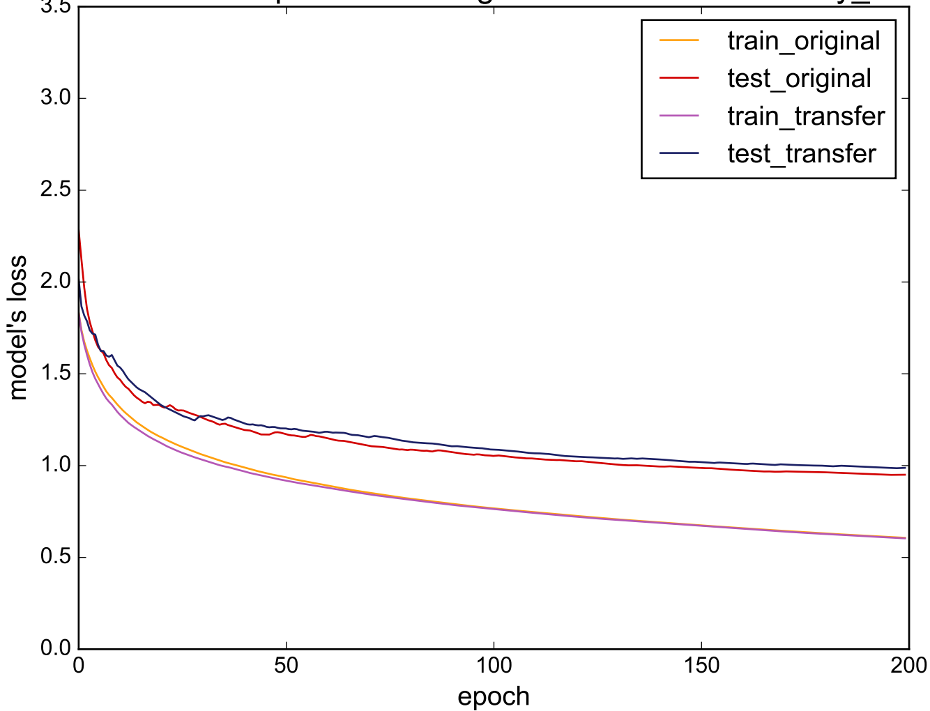
Source: ShapeletSim - Target: uWaveGestureLibrary_X
