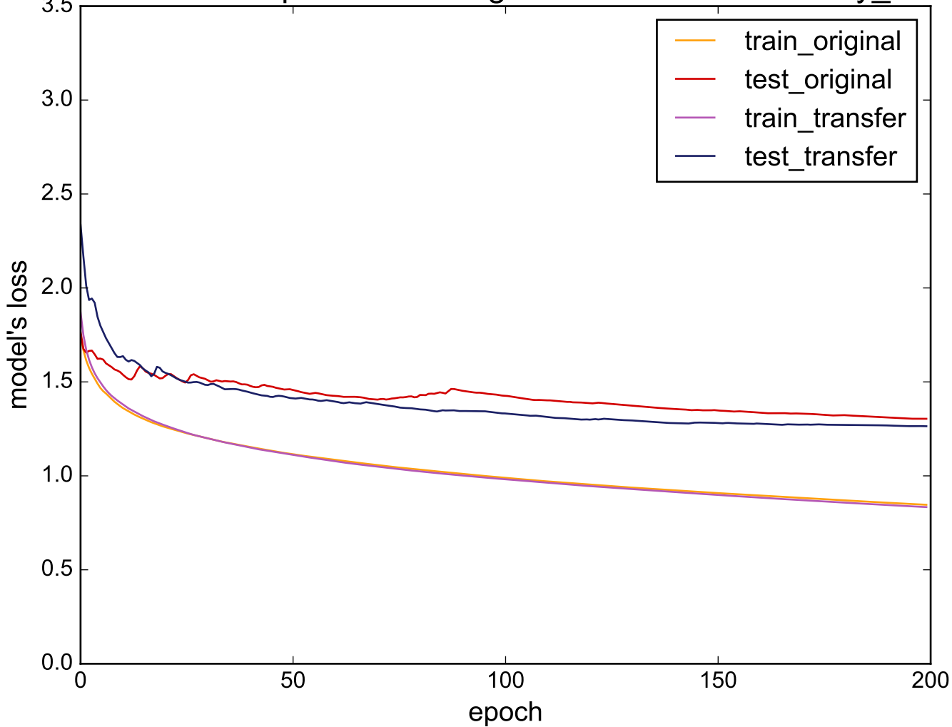
Source: ShapeletSim - Target: uWaveGestureLibrary_Y
