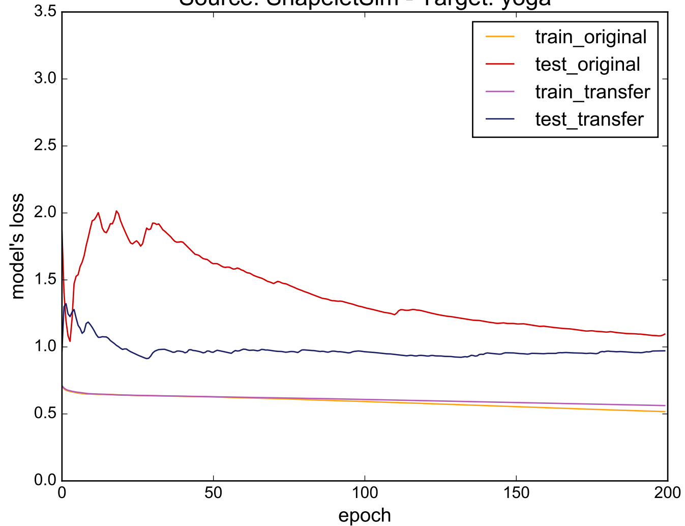
Source: ShapeletSim - Target: yoga
