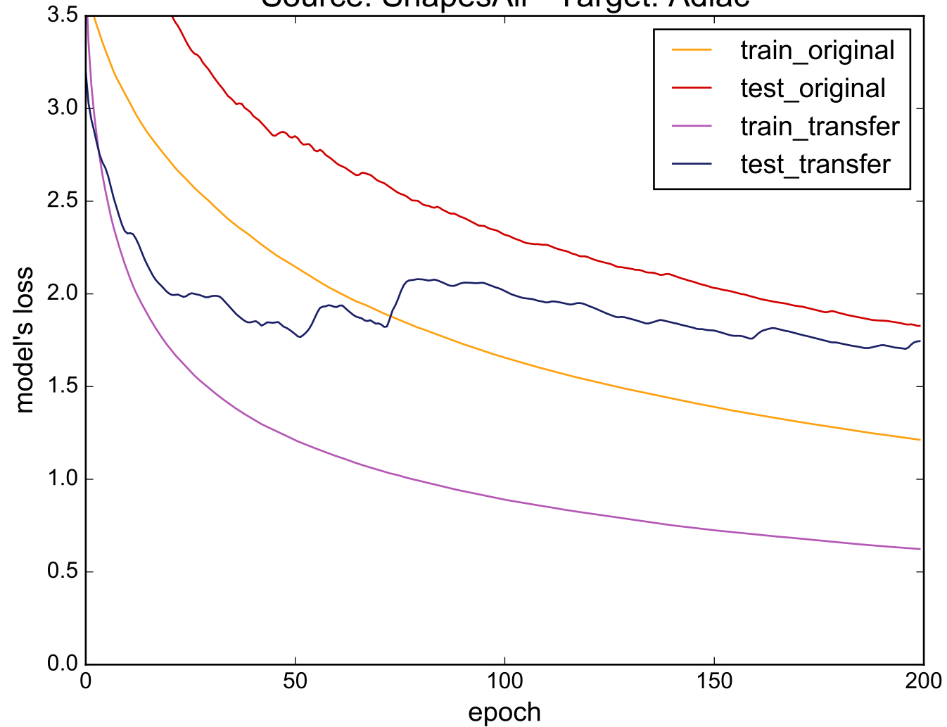
Source: ShapesAll - Target: Adiac
