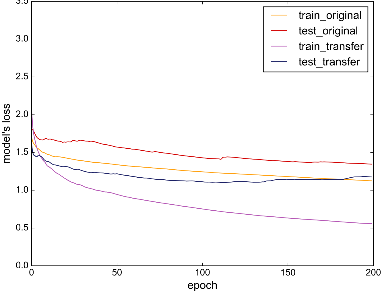
Source: ShapesAll - Target: Beef
