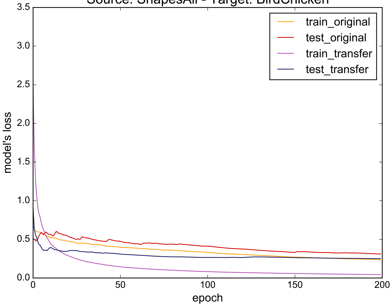
Source: ShapesAll - Target: BirdChicken
