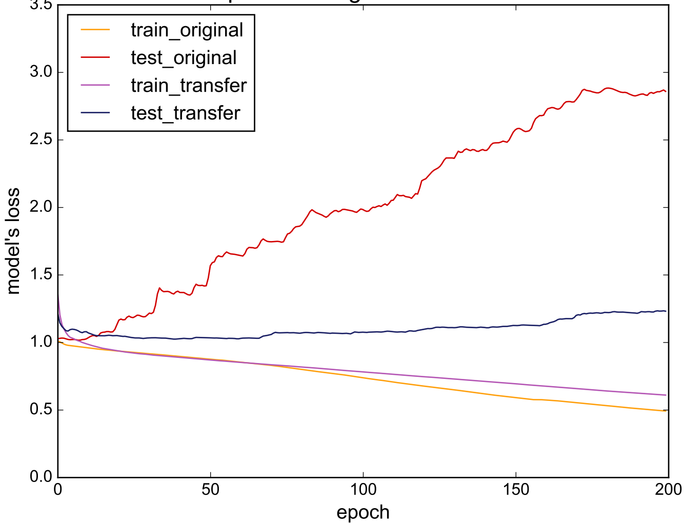
Source: ShapesAll - Target: ChlorineConcentration
