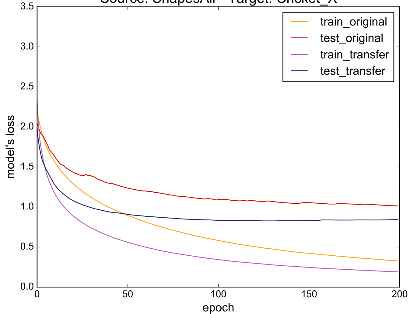
Source: ShapesAll - Target: Cricket_X
