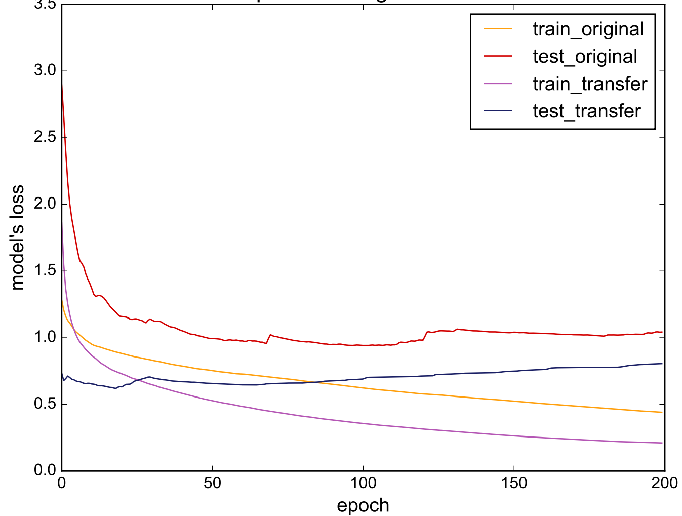
Source: ShapesAll - Target: DistalPhalanxTW
