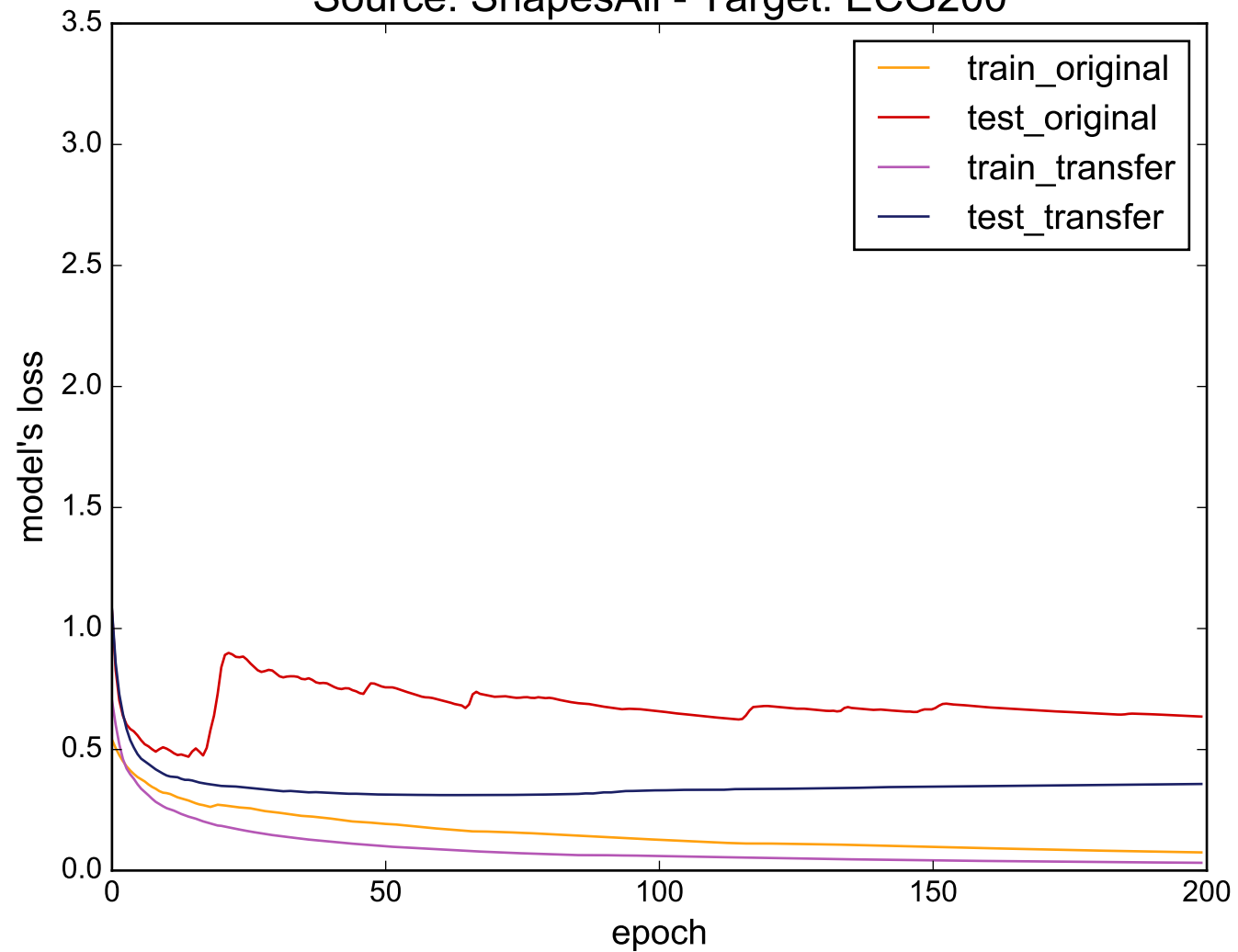
Source: ShapesAll - Target: ECG200
