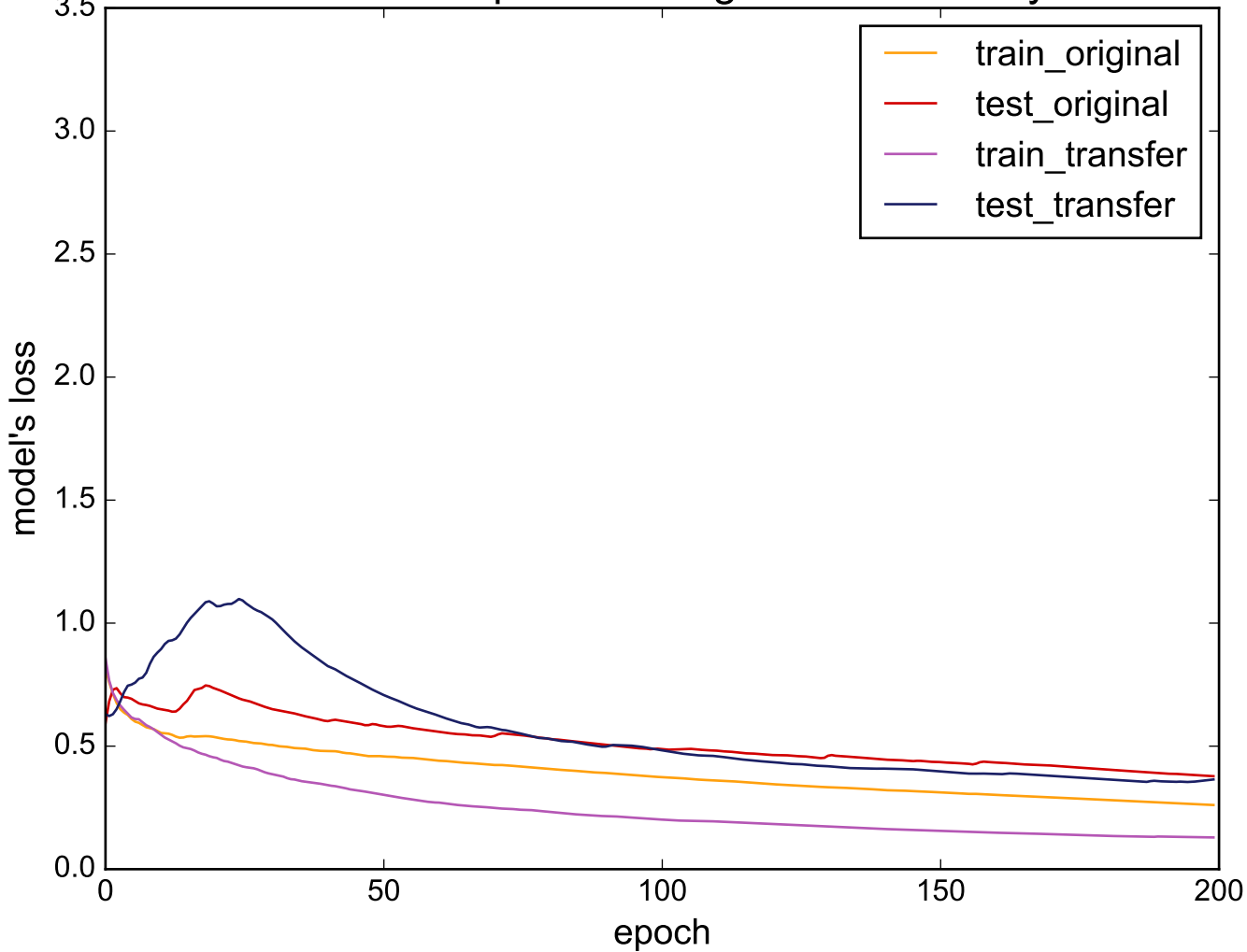
Source: ShapesAll - Target: ECGFiveDays
