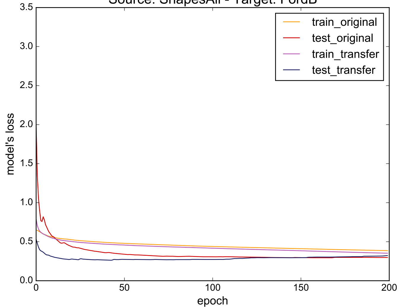
Source: ShapesAll - Target: FordB
