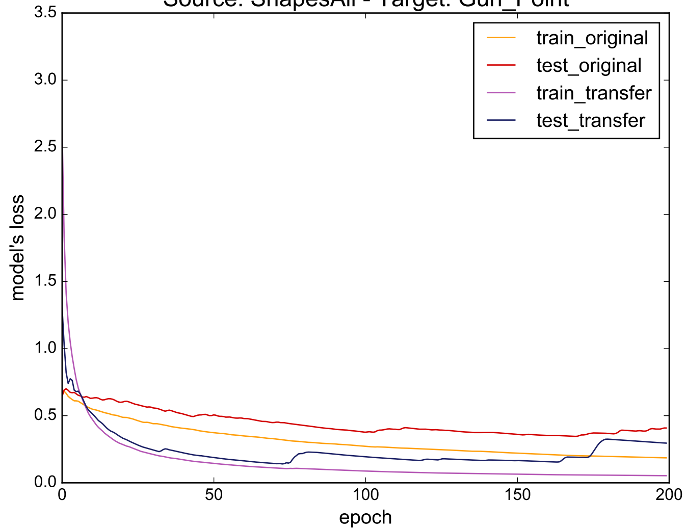
Source: ShapesAll - Target: Gun_Point
