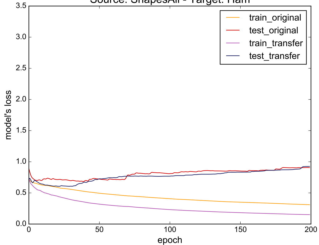
Source: ShapesAll - Target: Ham
