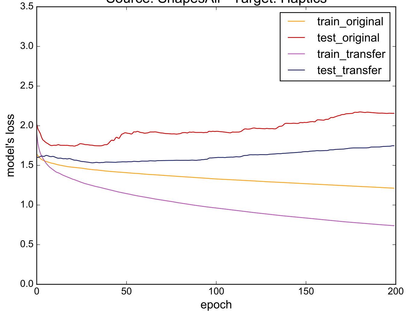
Source: ShapesAll - Target: Haptics
