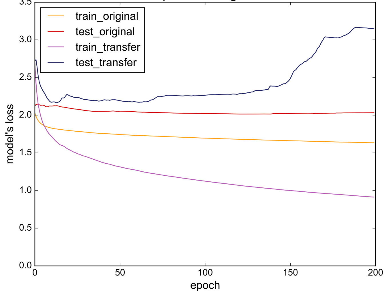
Source: ShapesAll - Target: InlineSkate
