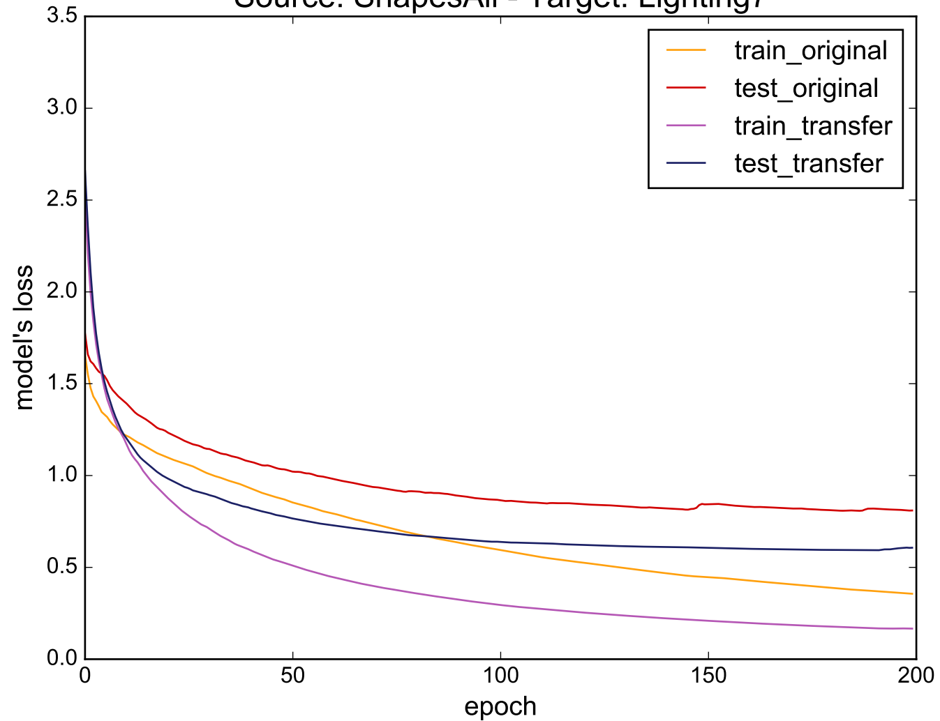
Source: ShapesAll - Target: Lighting7
