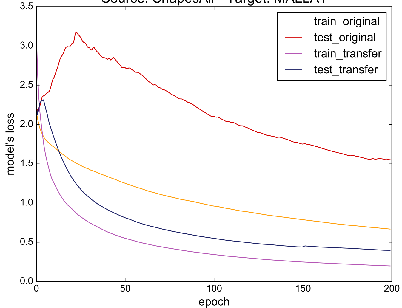
Source: ShapesAll - Target: MALLAT
