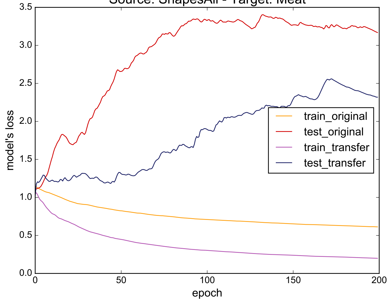
Source: ShapesAll - Target: Meat
