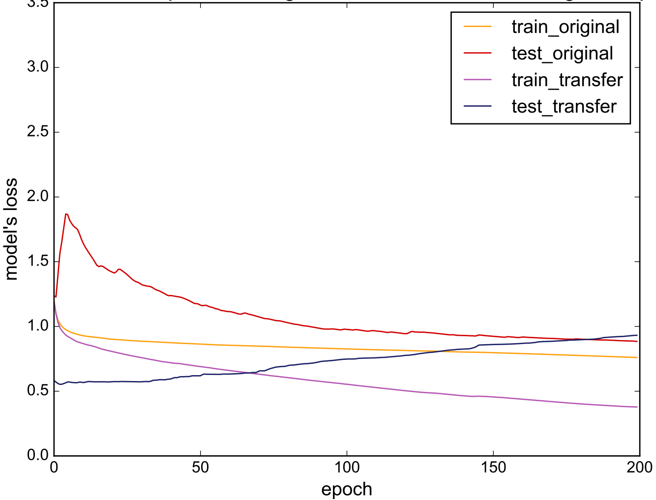
Source: ShapesAll - Target: MiddlePhalanxOutlineAgeGroup
