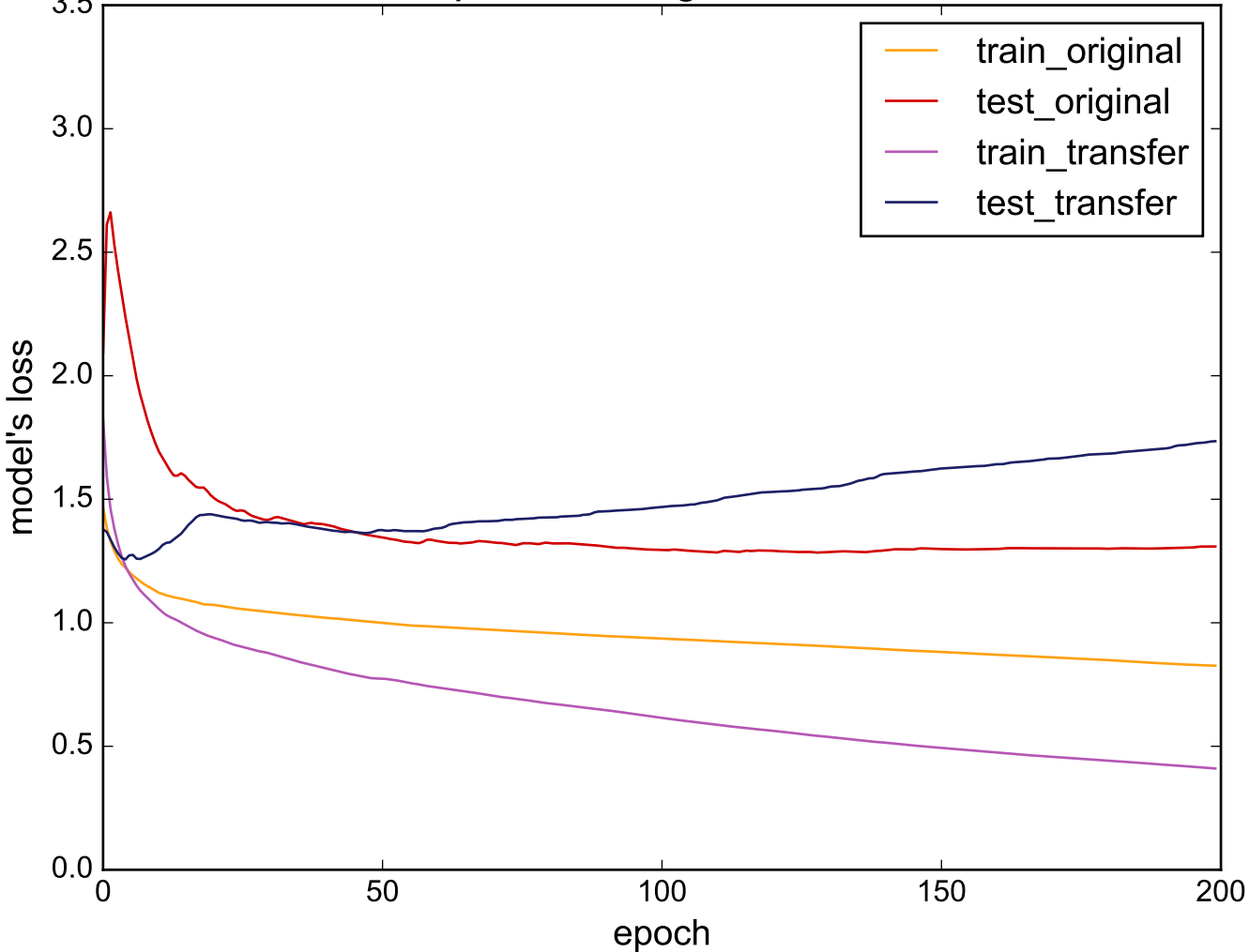
Source: ShapesAll - Target: MiddlePhalanxTW
