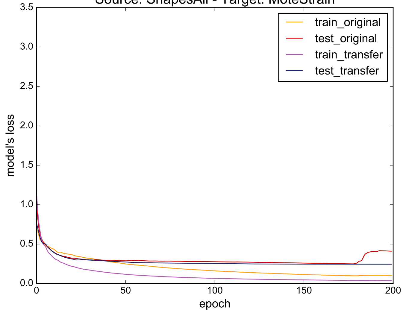
Source: ShapesAll - Target: MoteStrain
