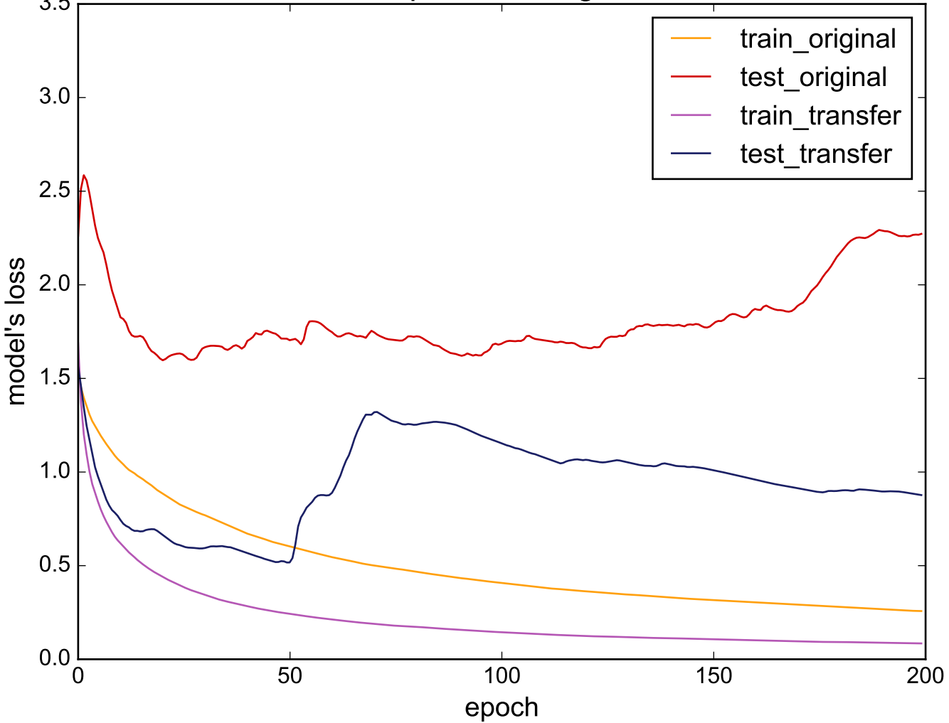
Source: ShapesAll - Target: OSULeaf
