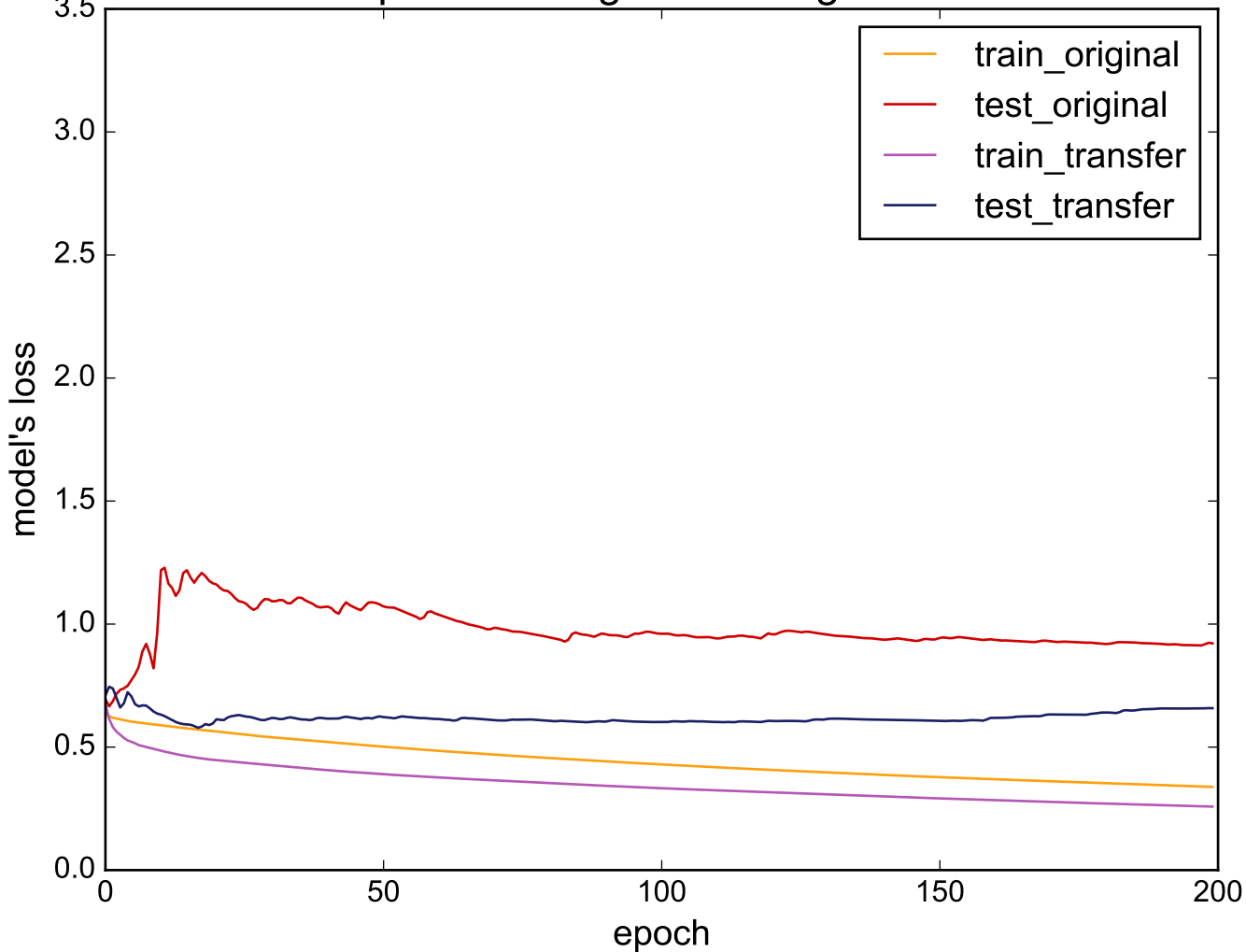
Source: ShapesAll - Target: PhalangesOutlinesCorrect
