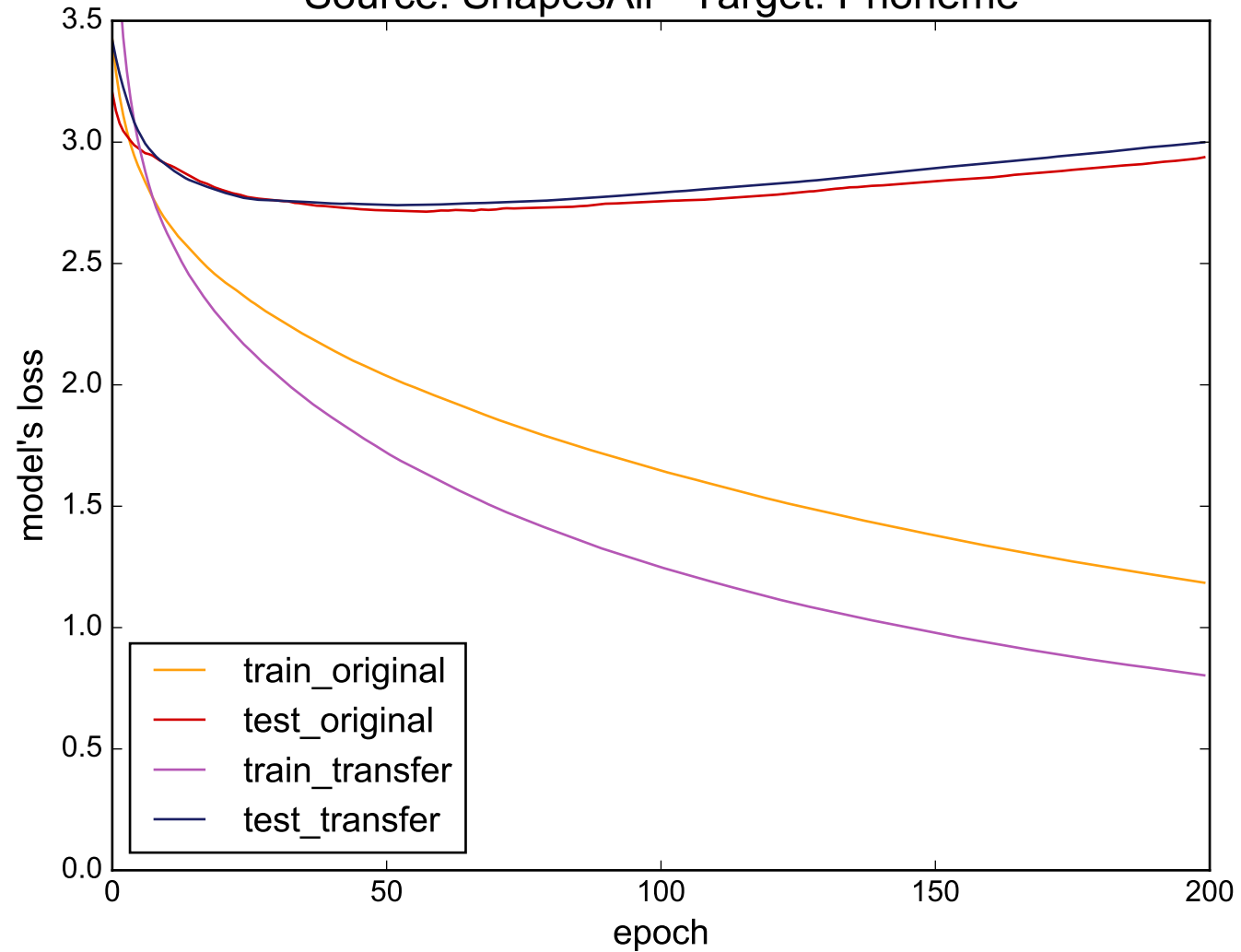
Source: ShapesAll - Target: Phoneme
