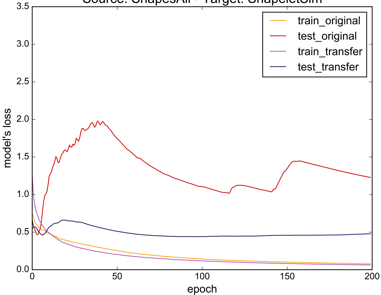
Source: ShapesAll - Target: ShapeletSim
