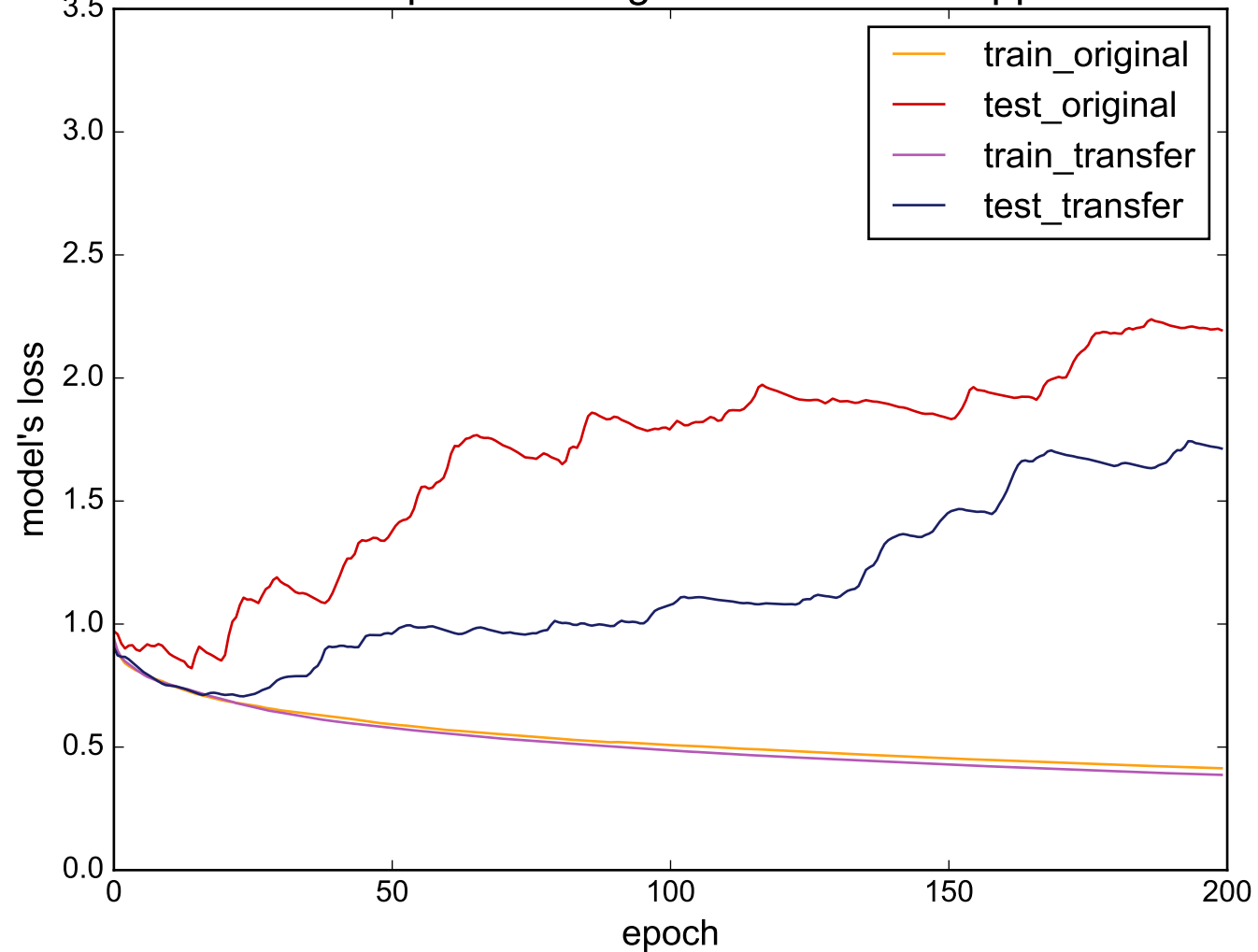
Source: ShapesAll - Target: SmallKitchenAppliances
