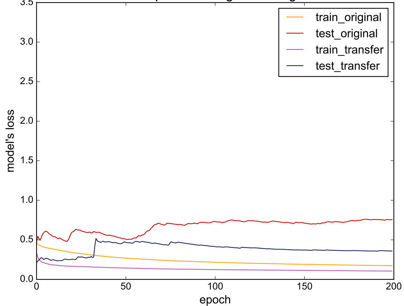
Source: ShapesAll - Target: StarLightCurves
