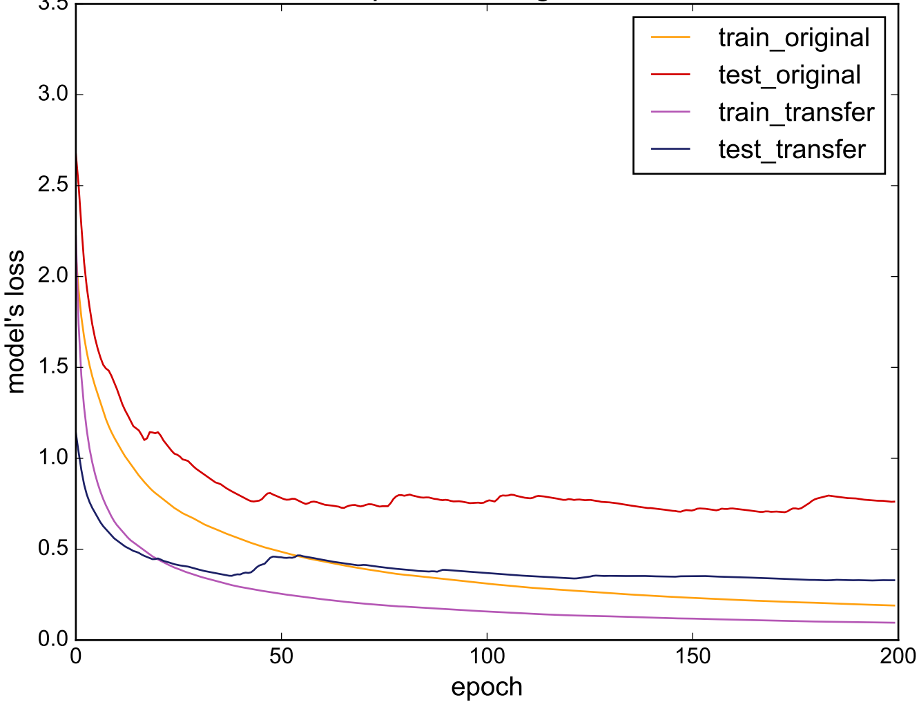
Source: ShapesAll - Target: SwedishLeaf
